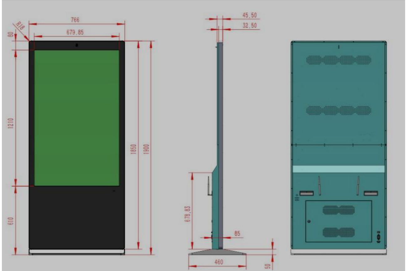
Machine dimensions Unit: mm
